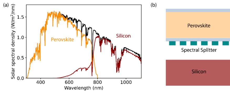
Figure 1 4T Perovskite/silicon tandem solar cell (a) Absorption of solar spectrum (black) in 500 nm thick perovskite top cell (orange) and silicon bottom cell (red) based on experimental data from [2]. (b) Schematic of air-coupled 4T tandem cell with spectral splitter metasurface on bottom side of perovskite top cell. Blue bands on top and bottom of the perovskite are glass layers (not to scale); the top glass is the superstrate for perovskite growth; the bottom glass layer supports the metasurface and is attached to the perovskite with index-matching oil.
