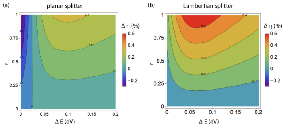
Figure S2 Parameter sweep of selective reflector step function for a (a) planar and (b) Lambertian spectral splitter in a 4T tandem solar cell with a top cell bandgap of E=1.55 eV and Si bottom cell.
