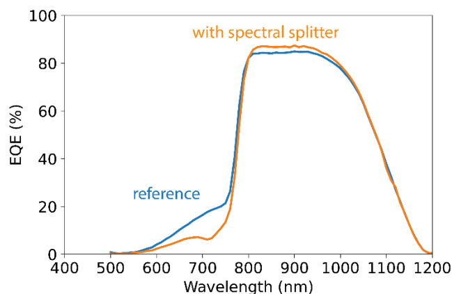
Figure S5 EQE measurement of Si bottom cell with and without spectral splitter.
