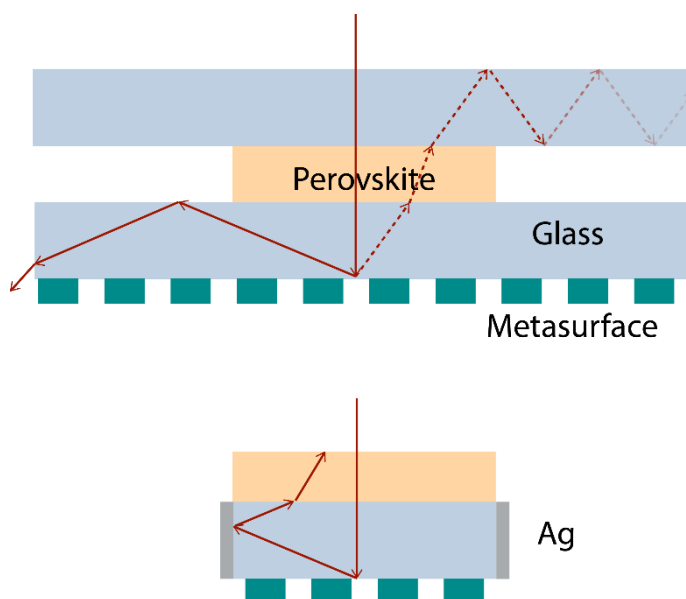
Figure S4 Schematic of edge effect in experiment. Top schematic: Part of the light escapes because the spectral splitter is bigger than perovskite cell (red solid line) and because the front glass slide is bigger than the perovskite cell (dashed red line). Bottom: If the spectral splitter is cut and the edges are covered with silver light is redirected to the perovskite cell
