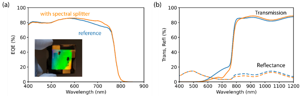
Figure 4 Measurements of metasurface integrated with perovskite cell. (a) EQE measurements of perovskite with spectral splitter (orange) and with glass reference (blue) Inset: Photograph of perovskite with spectral splitter taken from the bottom (facing the metasurface). Diffracted colors from the metasurface are clearly visible. (b) Transmission and reflectance measurement of the perovskite cell with spectrum splitter integrated.
