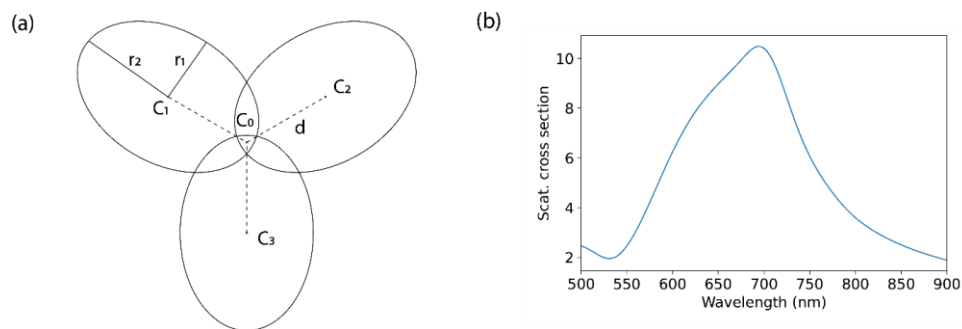
Figure 3 (a) Dimensions of the windmill shaped a-Si:H particle in the hexagonal unit cell of the metagrating. (b) Scattering cross section of the optimized particle.
