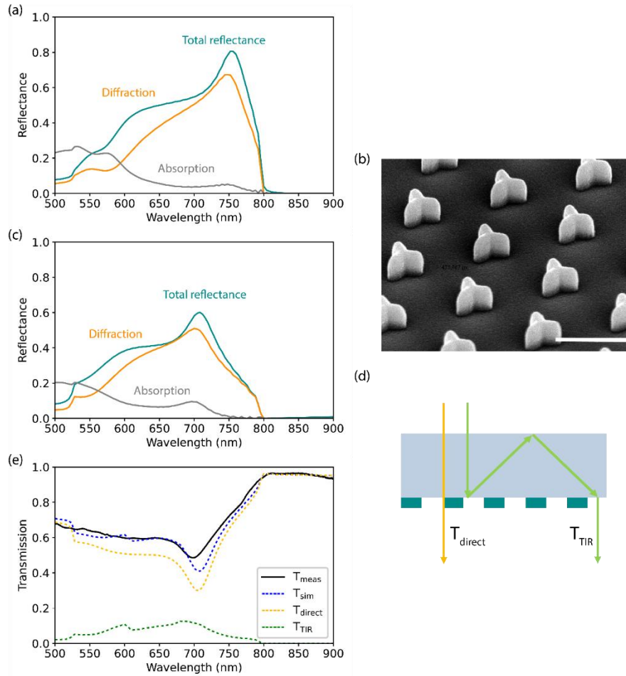
Figure 3 Spectral splitter metasurface. (a) Simulated total reflectance (green), diffraction (orange) and absorption (grey) of optimized spectral splitter metasurface. (b) SEM tilted top-view image of metasurface: a-Si:H windmill shaped particles on glass substrate (covered with around 10 nm chromium layer for better imaging). Scale bar is 500 nm. (c) Simulated total reflectance (green), diffraction (orange) and absorption (grey) of fabricated spectral splitter metasurface. (d) Paths of transmission through glass slide with same coloration as in (e). (e) Optical transmission measurements (black) of fabricated metasurface, calculated/simulated transmission (blue dashed line) composed of direct transmission (yellow dashed line) and transmission after total internal reflection (green dashed line).
