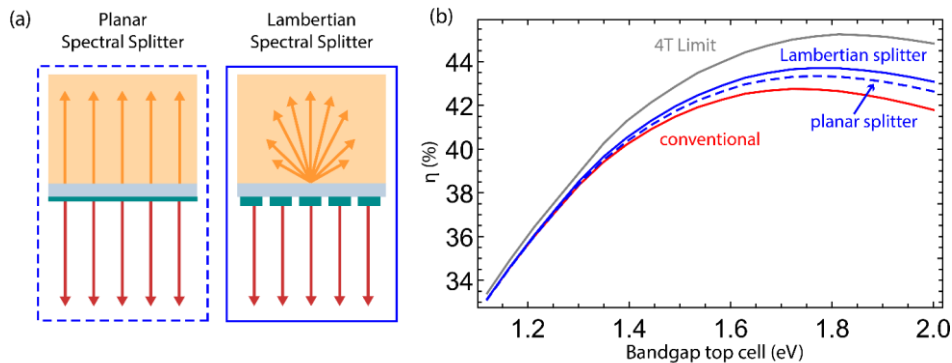
Figure 2 Spectral splitting in 4T tandem cell. (a) Schematics of planar (left) and Lambertian (right) spectral splitter. (b) Efficiency limit from detailed balance calculations of 4T tandem cell as function of top cell bandgap energy with silicon bottom cell ( E_{BG}=1.12 \text{ eV} ). Thermodynamic limit (gray line), limit for 580 nm thick perovskite top cell (red line) and 580 nm thick perovskite top cell with integrated planar (dashed blue line) and Lambertian spectral splitter (solid blue line).
